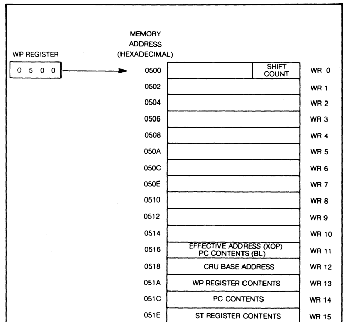
Figure 1. Reserved Areas of 9900 Workspaces
