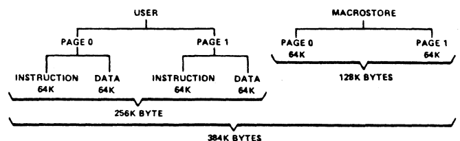
FIGURE 12 – TMS 99000 EXTENDED ADDRESSING
