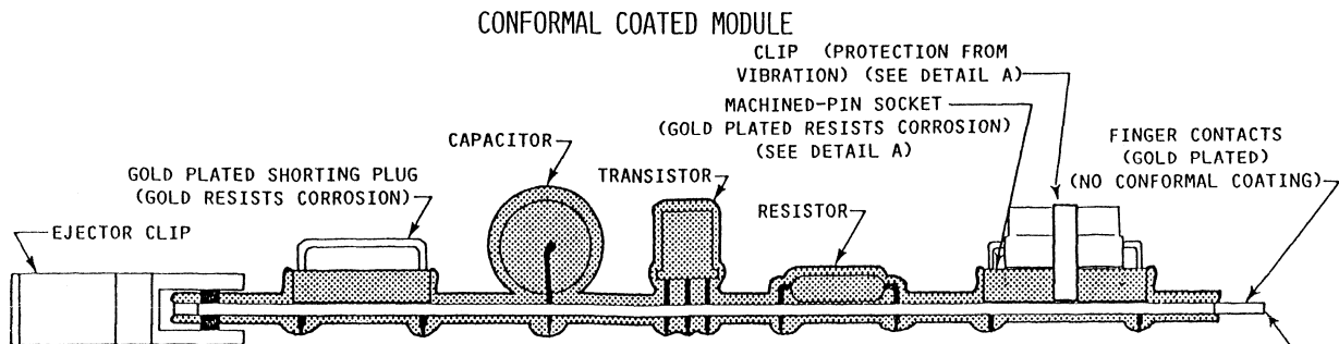
SIDE VIEW OF TM 990 MODULE
