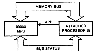
FIGURE 9 – ATTACHED PROCESSOR/COMPUTER INTERFACE
