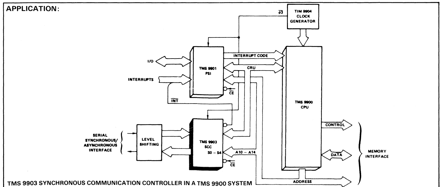
TMS 9903 SYNCHRONOUS COMMUNICATION CONTROLLER IN A TMS 9900 SYSTEM
