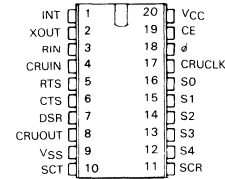
TMS 9903 PIN ASSIGNMENTS 20 PIN DUAL-IN-LINE PACKAGE (TOP VIEW)
