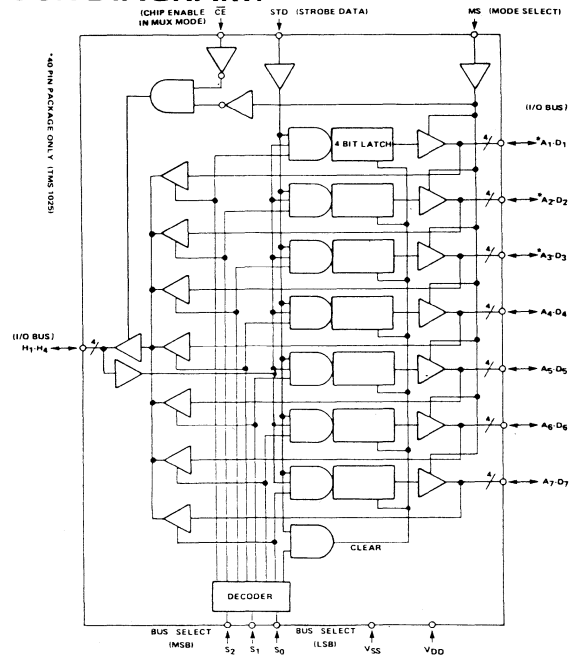
INPUT EXPANSION USING THE TMS 1025
